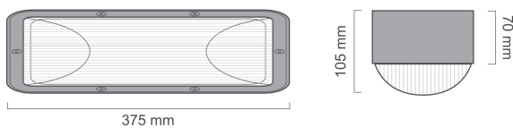
Dish Diffuser
